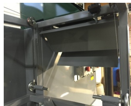
Detail of adjustable distribution chute
