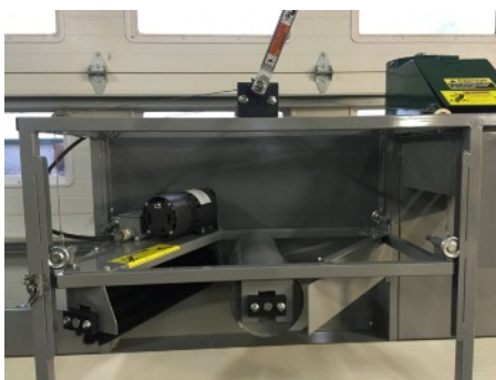
Detail of leveling roller and brush assembly
